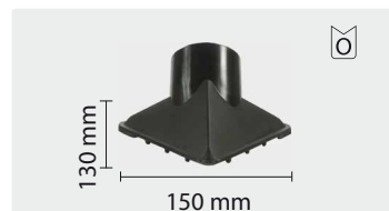
tobera triangular
